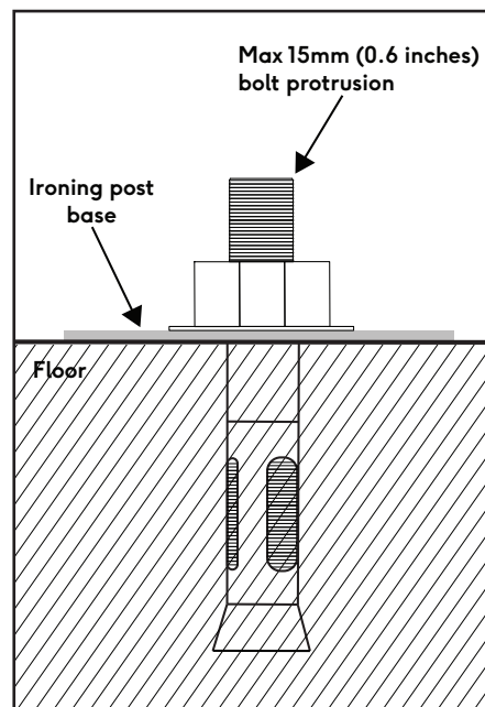
Fig 1 M16/95mm galvanised sleeve anchor
