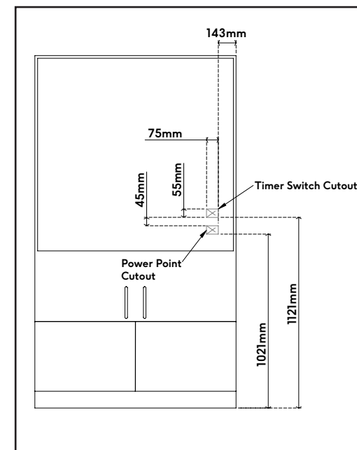
Fig 2 Electrical rough in details for full size unit (not trim version)
