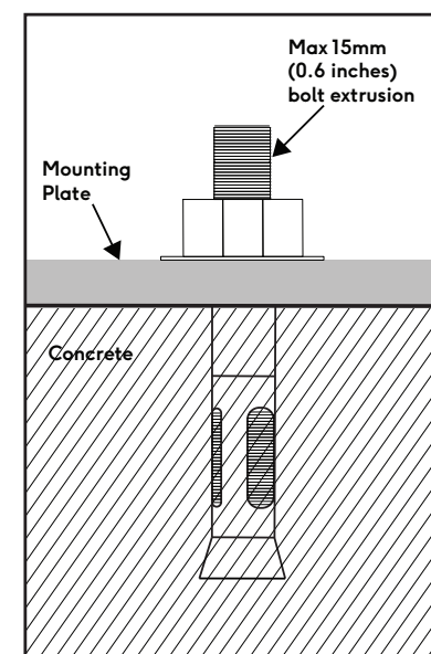
Fig 5/ Silver Bullet Fixing
