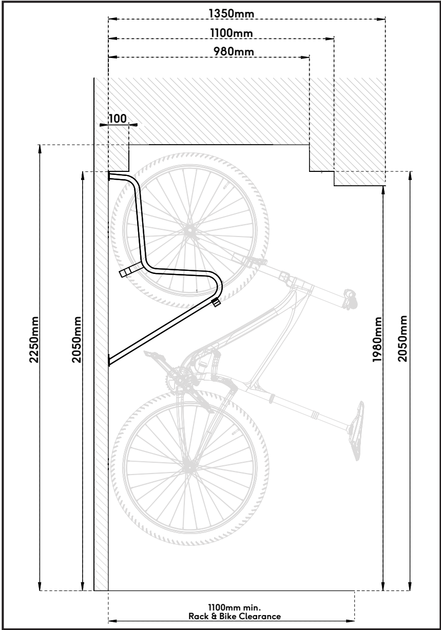
Cradle Clearance Map - Path Of Travel
