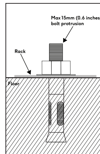
Fig 2 M10x75mm (3/8" x 3") sleeve anchor (dynabolt)
