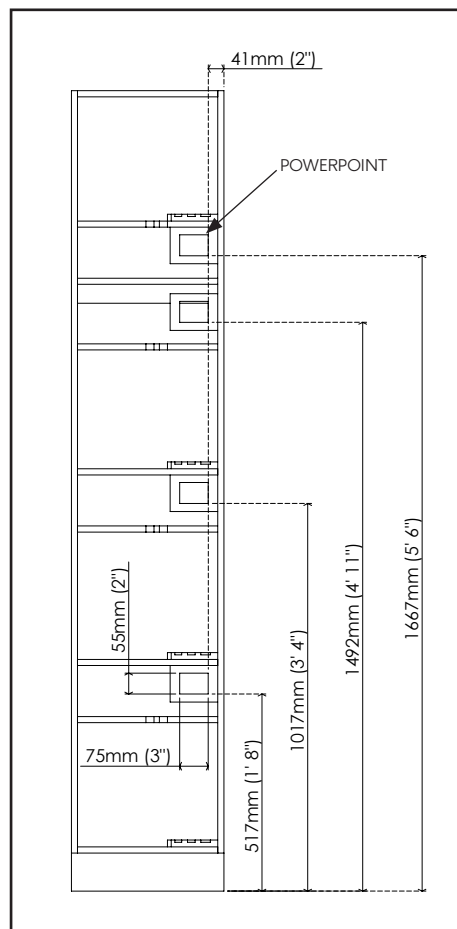
Fig 1 Electrical rough in detail
