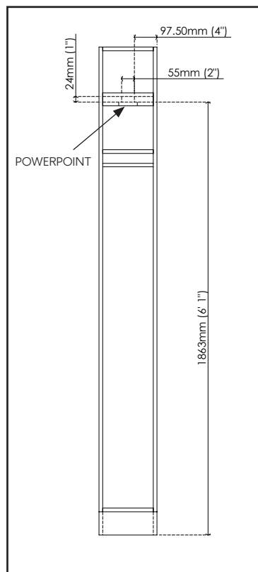
Fig 1 Electrical rough in detail
