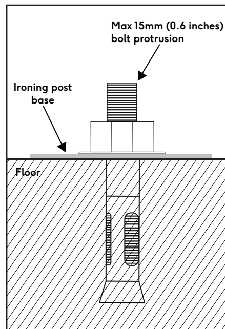
Fig 1 M16/95mm (25/64" x 3 47/64") galvanised sleeve anchor
