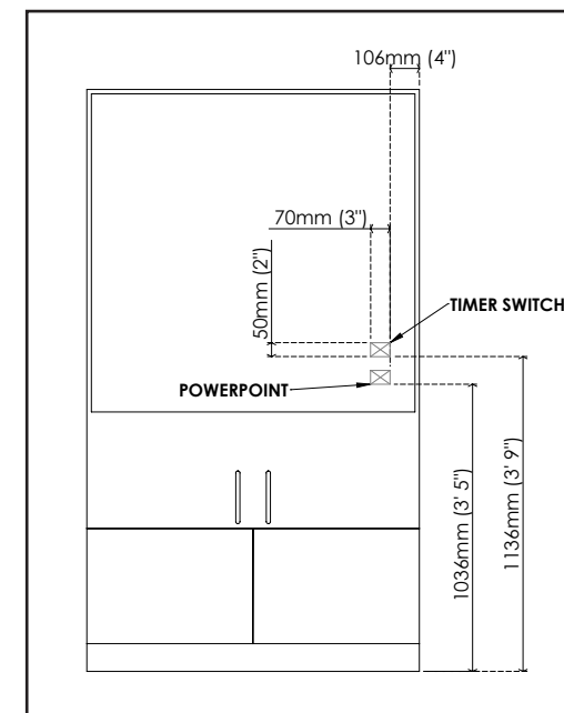
Fig 2 Electrical rough in details
